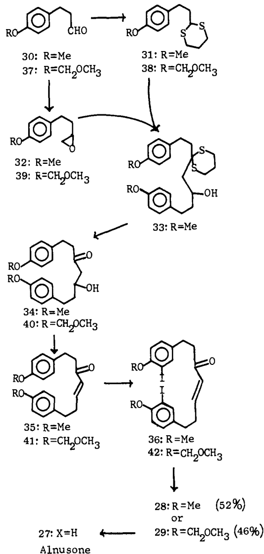
Figure 3. Synthesis of alnusone.
