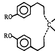
Figure 2. Strategy for alnusone.
